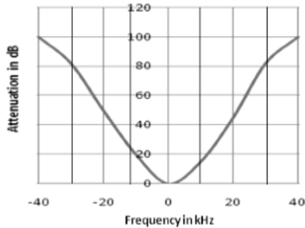
Fig1. Selectivity curve
